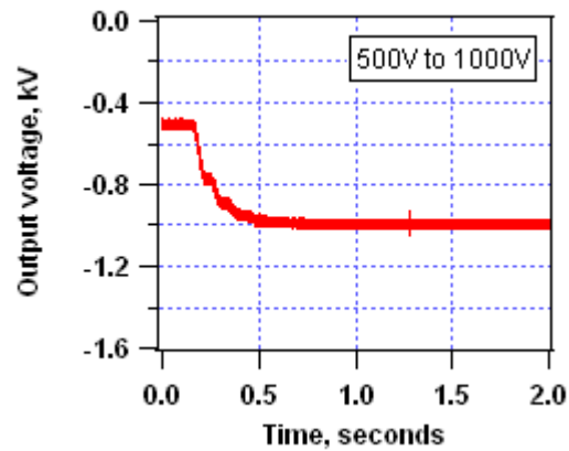
Figure 5: Turn-on behavior. Response to a step on Vctrl from -500V to -1000V output.
