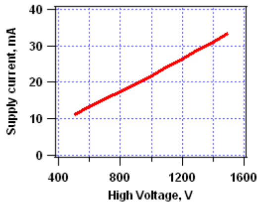
Figure 2: The supply current current is proportional to the high voltage: about 21mA/kV.
