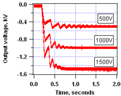
Figure 4: Turn-on behavior. Response to a step on Vctrl for a 0V to 500V, 1000V and 1500V step.
